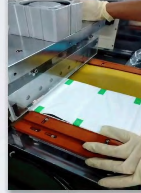
Tab cutting
