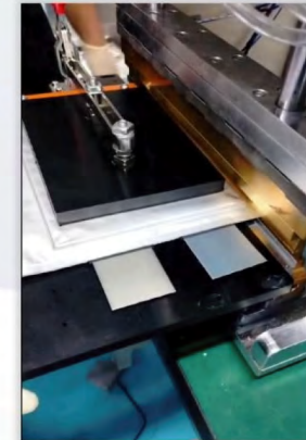
Side sealing
